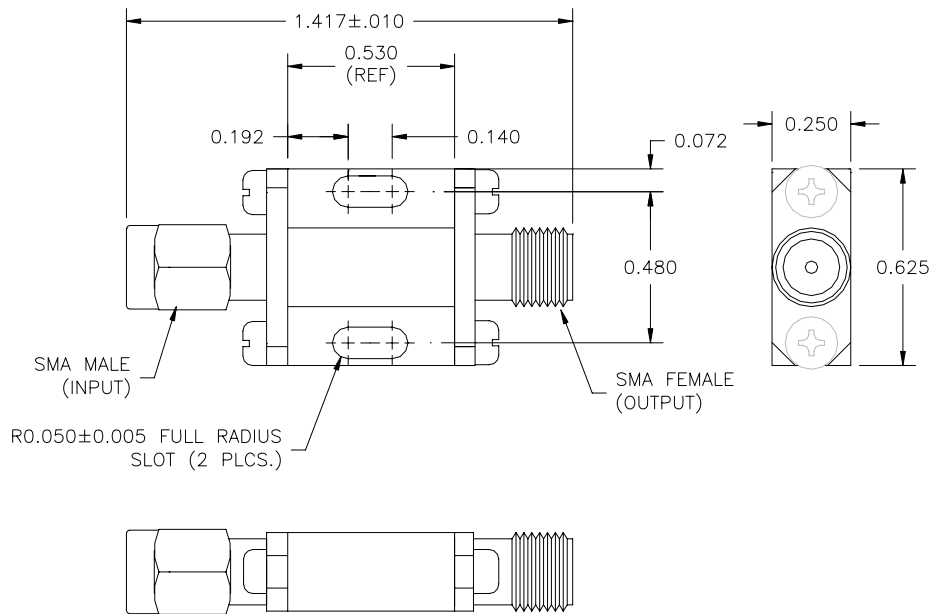
STANDARD CASE STYLE C36 (Optional Case Styles – C37, M61)
